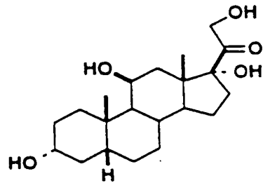
Tetrahydrocortisol (THF)
